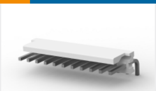
TE Part # 1-640389-1 11P MTA156 HDR ASSY SQ R/A F/L
